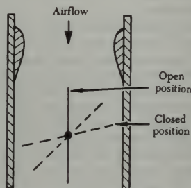
FIGURE 3-5. Throttle action.
